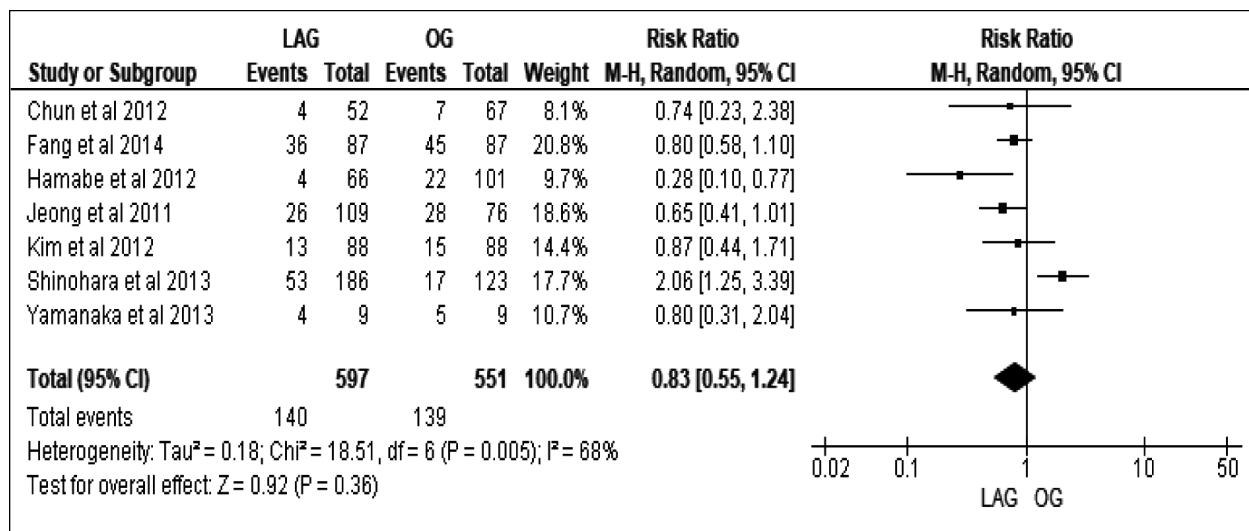
Figure 3: Recurrence rate.
